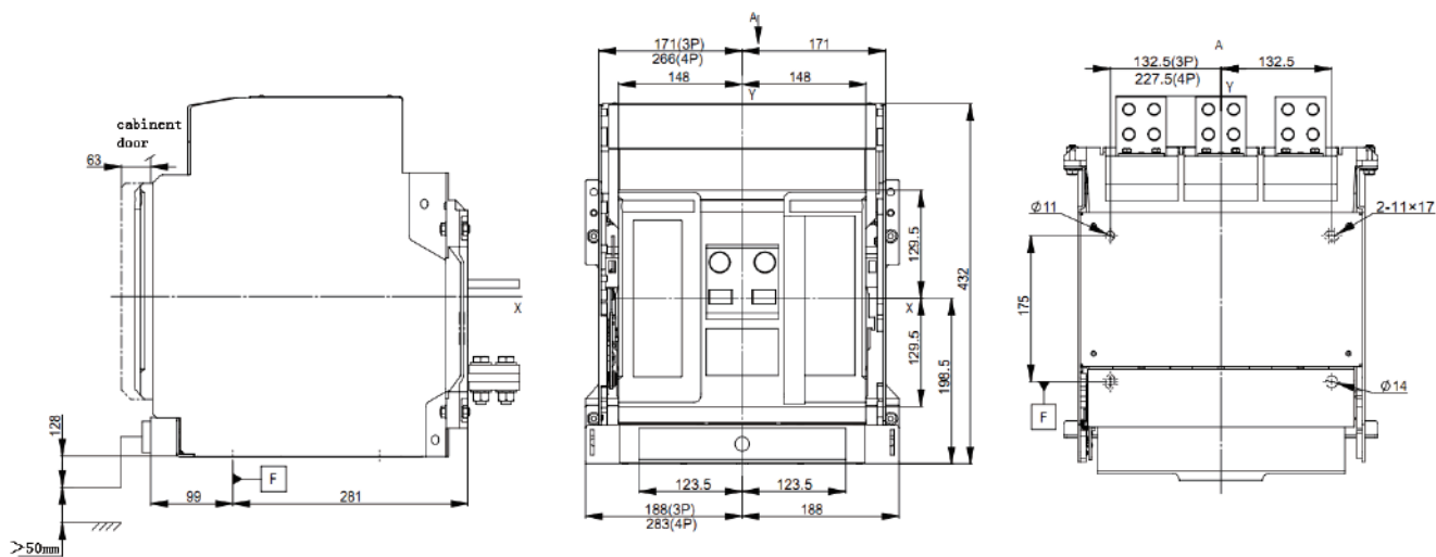
Fixed Details
