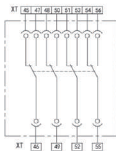
Four groups switch JDA-W2G-2000/4000
