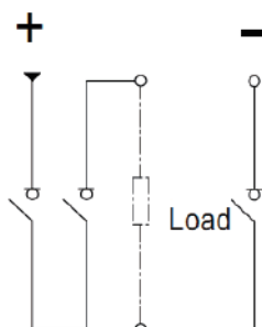
Type B Wiring Method
