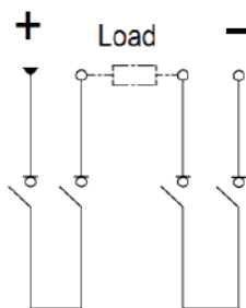
Type C Wiring Method
