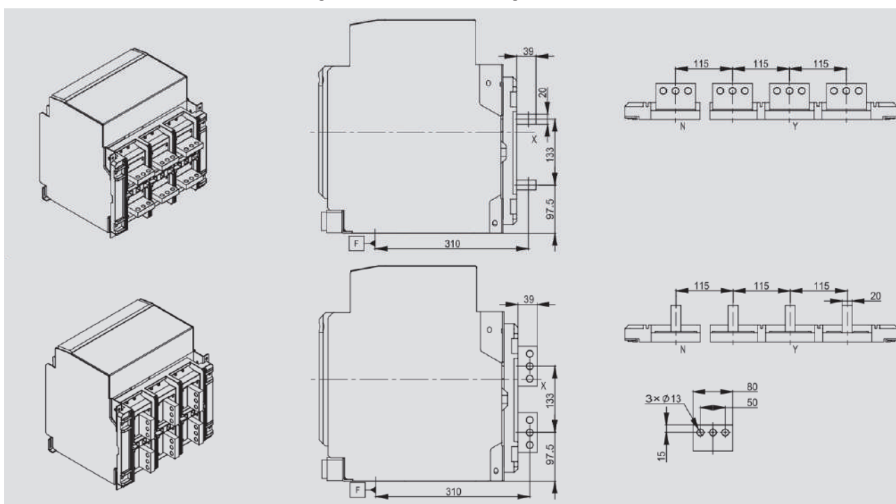
800A-2500A Horizontal Extended Wiring, Vertical Extended Wiring
