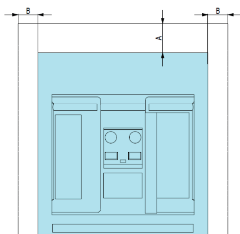
Drawout disconnecting switch
