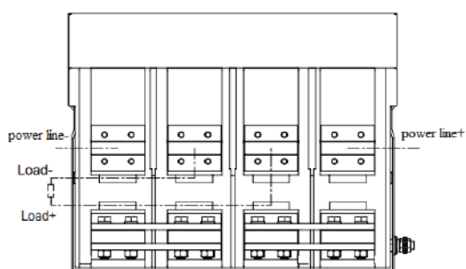
Type C Wiring Method
