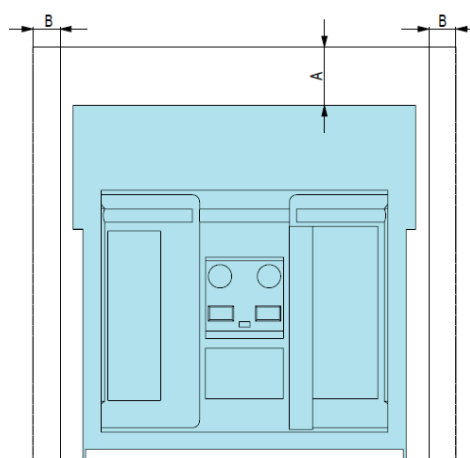
Fixed disconnecting switch
