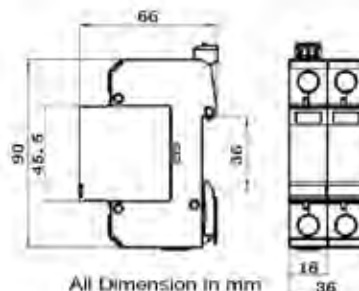
Dimension drawing
