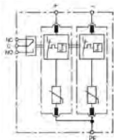
Basic circuit diagram
