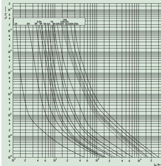
CH 10 gPV I/t characteristics
