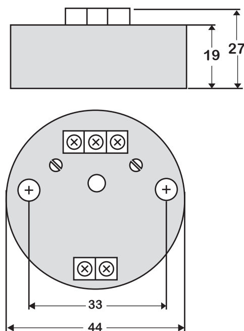
DIMENSIONS(mm)
