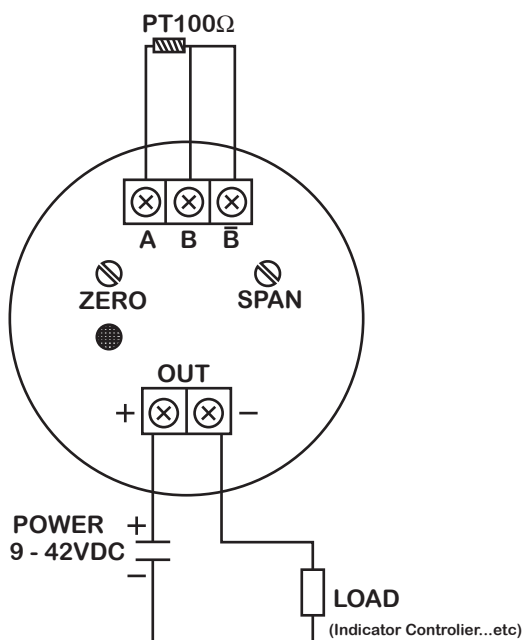
CONNECTION DIAGRAM
