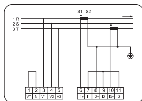
Unbalanced 3-phase, 3 wires + 2 CTs
