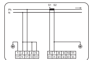
Single-phase connection
