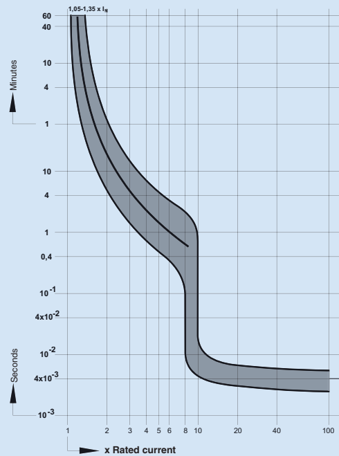
G characteristic I_n = 12 - 60 \text{ A} UL
