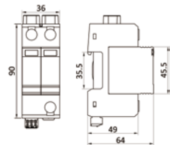
Dimension drawing
