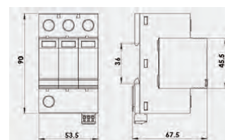
Dimension drawing
