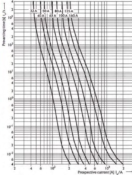
NH DC 750V, 1000V t-I characteristics
