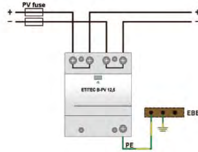
V - Connection ETITEC B-PV
