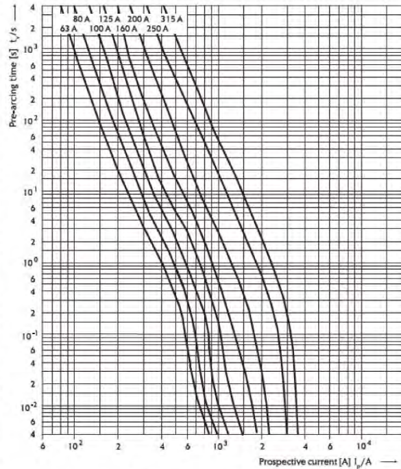
NH DC 1100V t-I characteristics
