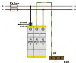
T connection ETITEC C-PV
