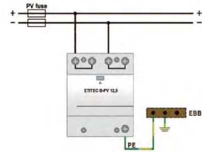
T - Connection ETITEC B-PV
