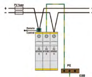
V connection ETITEC C-PV
