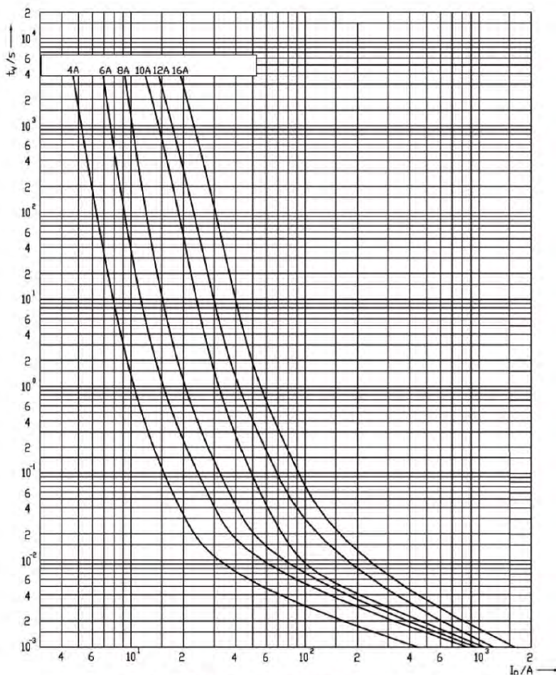
CH 10 PV t-I characteristics
