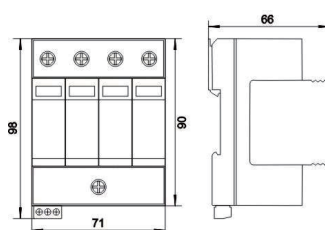
Dimension drawing
