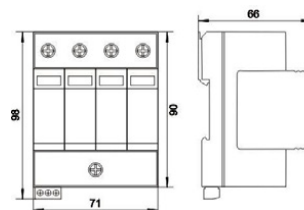
Dimension drawing
