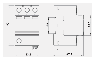
Dimension drawing
