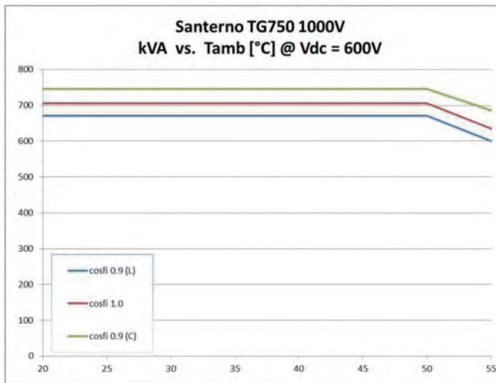
Figure 4: Temperature derating (installation altitude below 1000mt)
