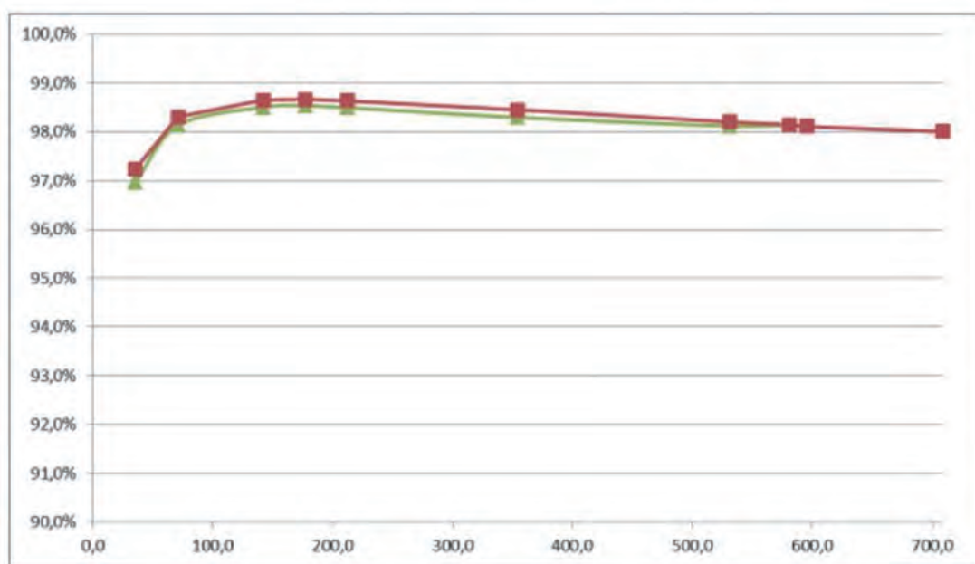
Efficiency Chart between 600Vdc and 820Vdc
