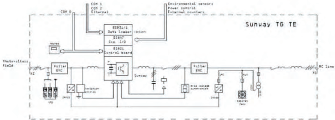
Figure 1: Block schematics
