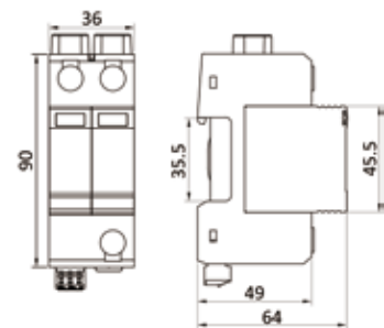
Dimension drawing
