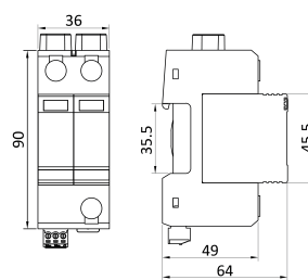
Dimension drawing
