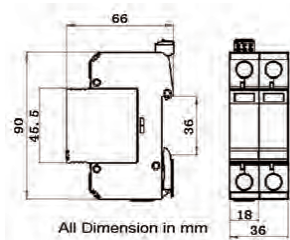
Dimension drawing
