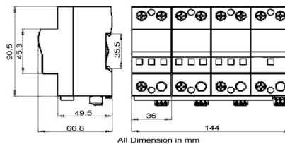
Dimension drawing
