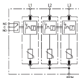
Basic circuit diagram
