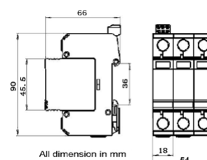
Dimension drawing
