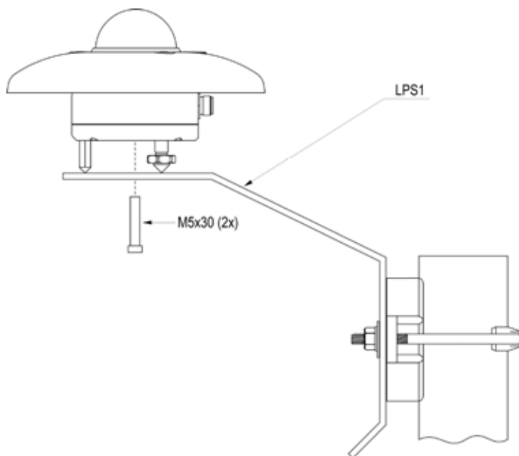
Fig. 4.2: LPS3 bracket for mast
