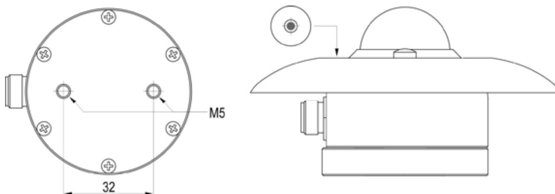
Fig. 4.1: position of fixing holes and bubble level
