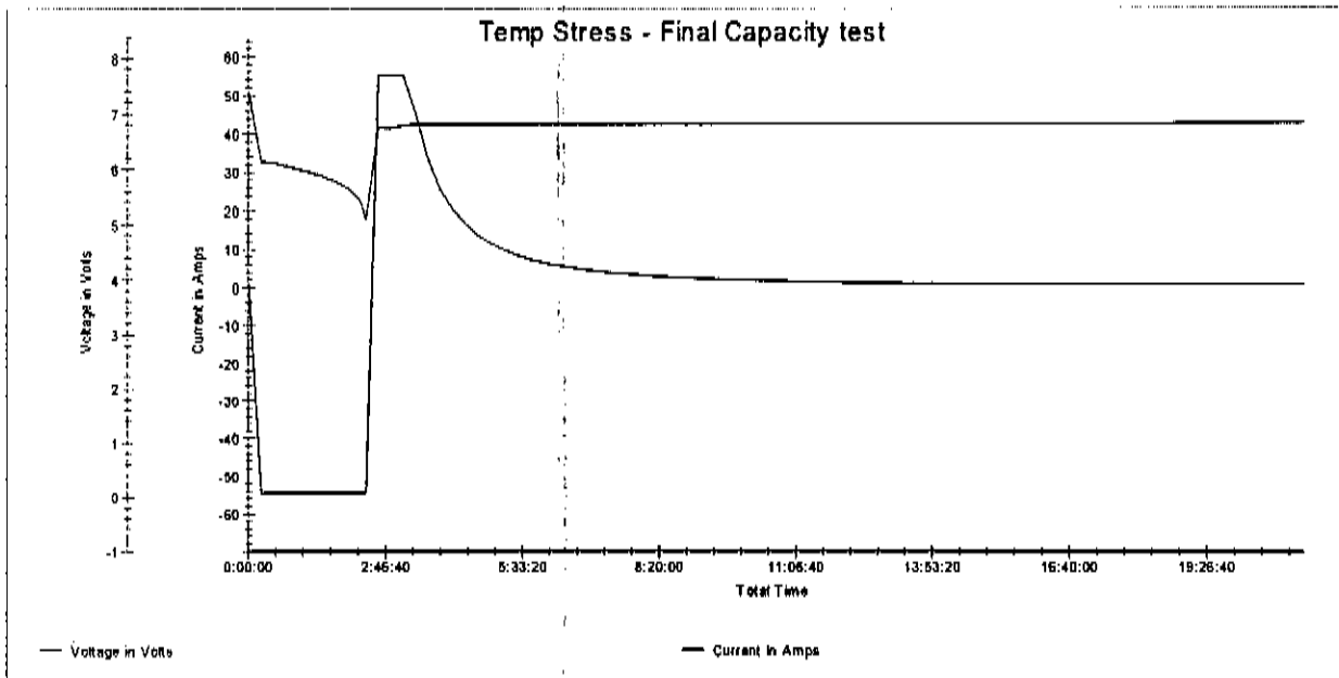
Graph of final capacity test on battery subjected to the Temperature Stress Test.
